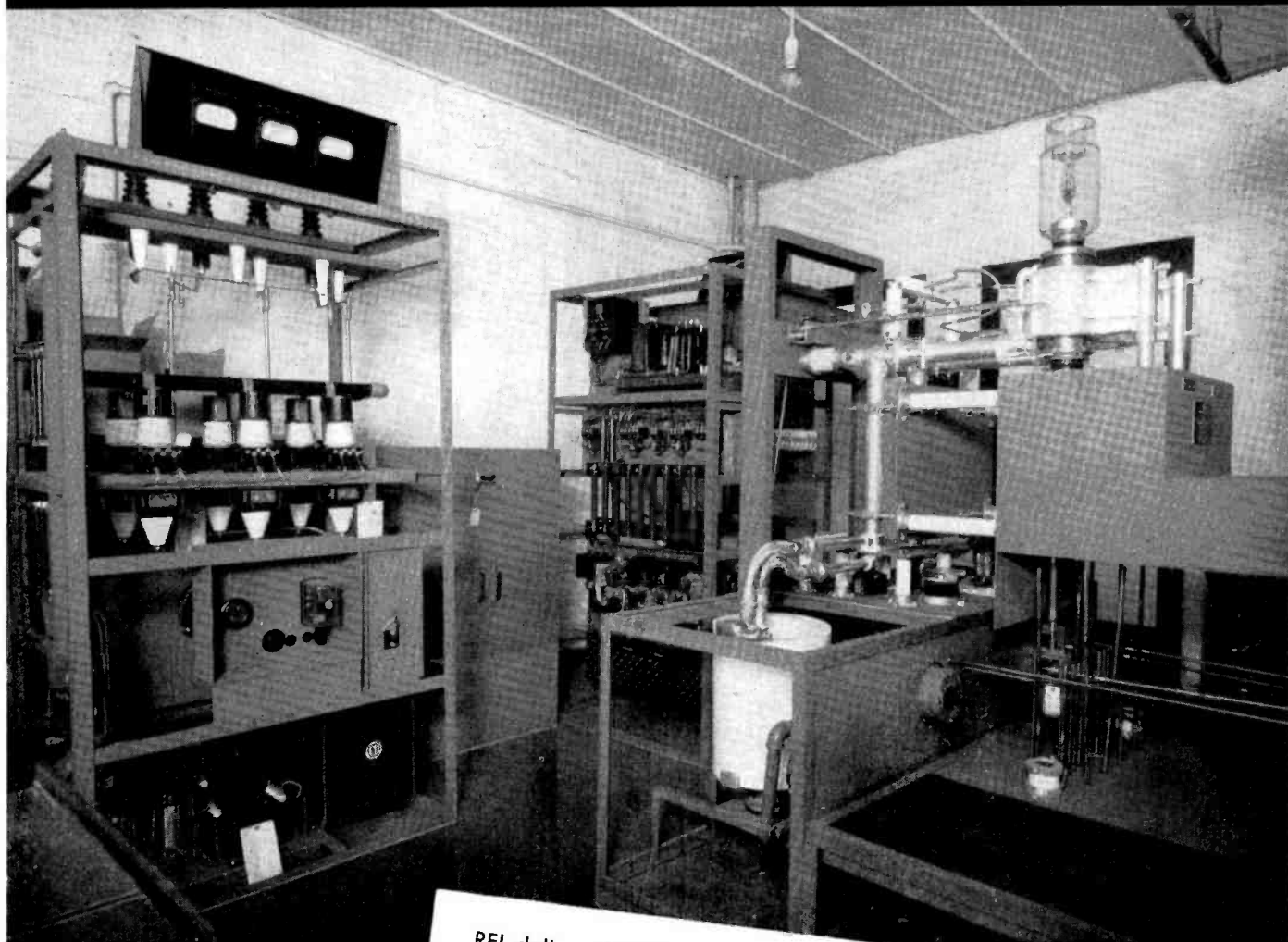
Photo of the REL 50 kw FM transmitter just completed and ready for delivery to W4SD, The Detroit Evening News.
